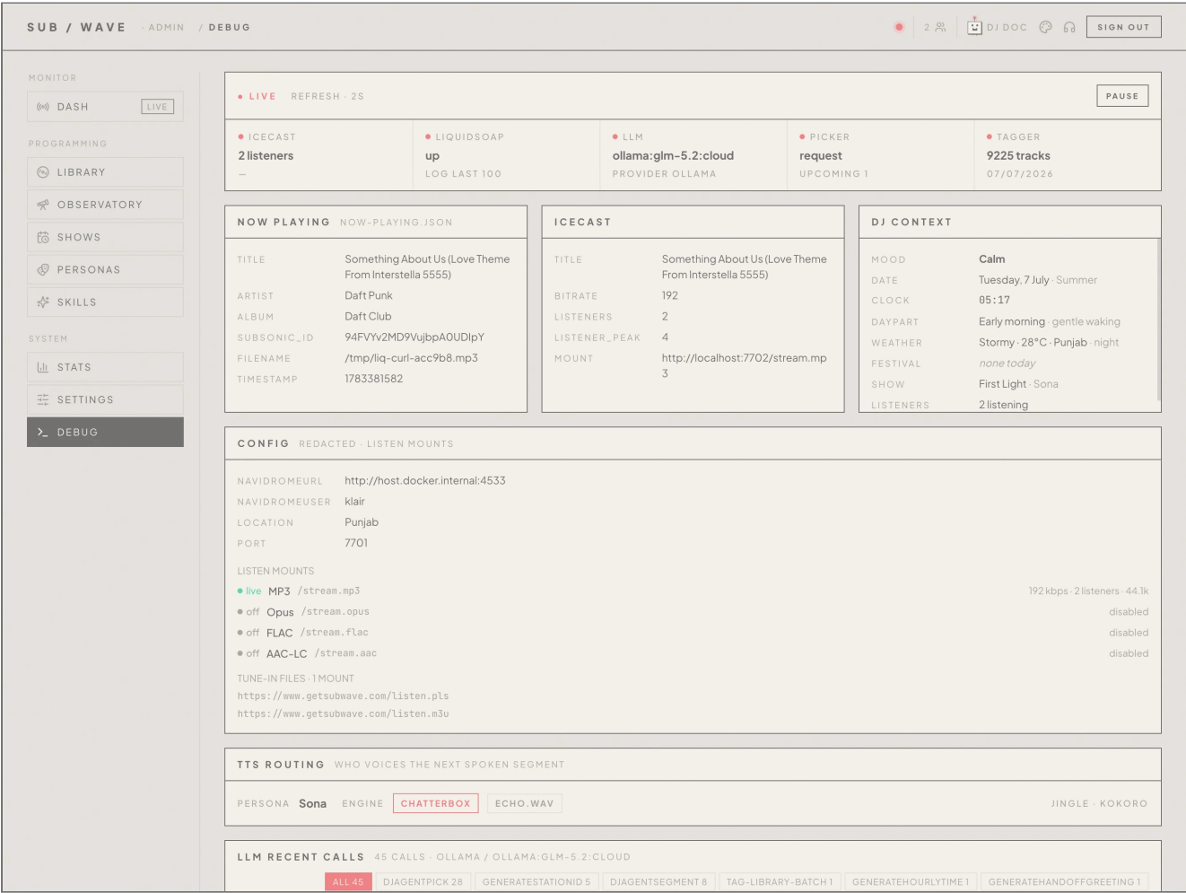
FIG. DEBUG: A HEALTH STRIP, LIQUIDSOAP LOGS, AND RECENT LLM CALLS, REFRESHED LIVE.
