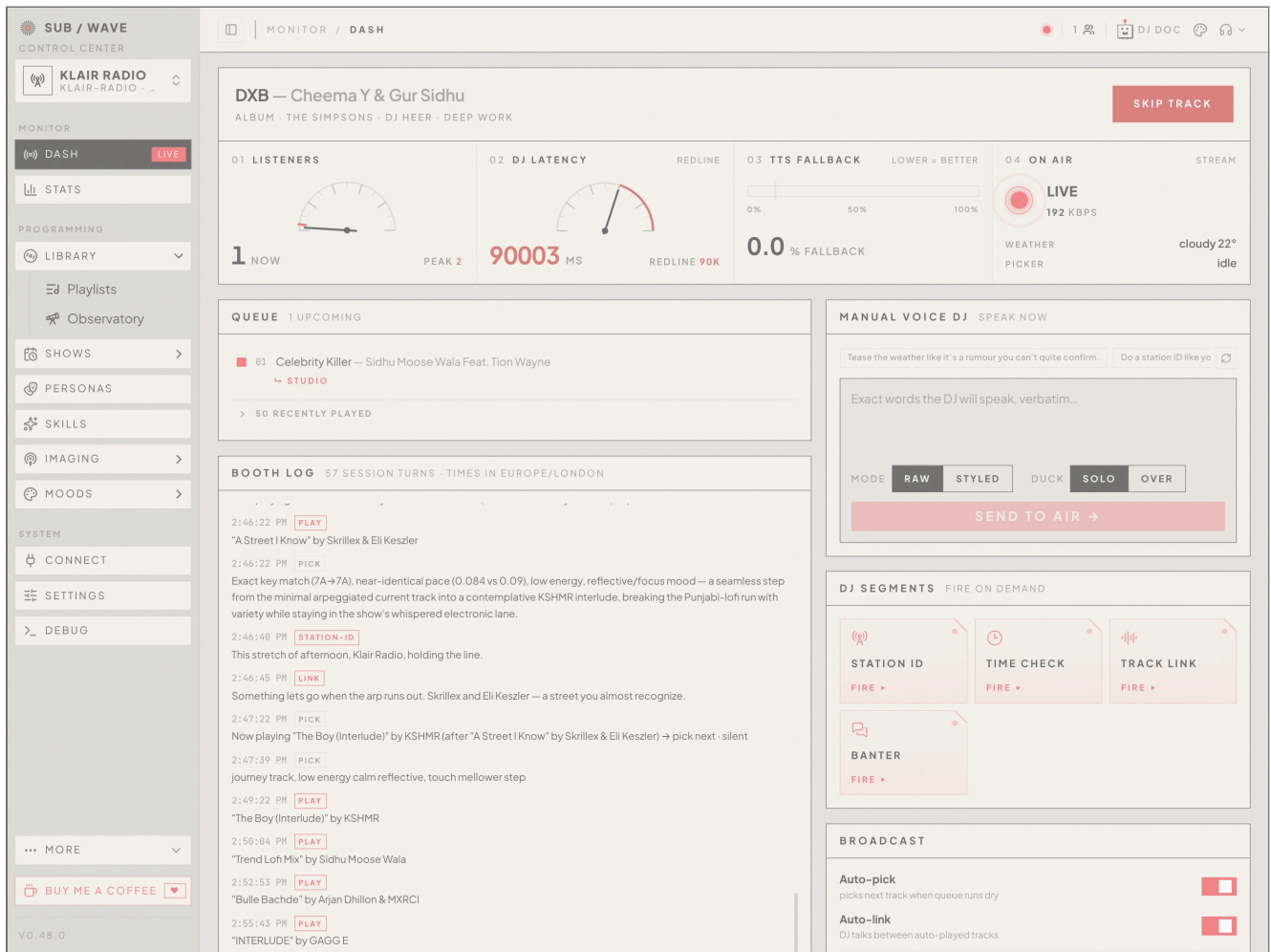
FIG. THE DASH PANEL: LIVE STATUS, THE QUEUE, THE BOOTH LOG, AND MANUAL VOICE CONTROL.
